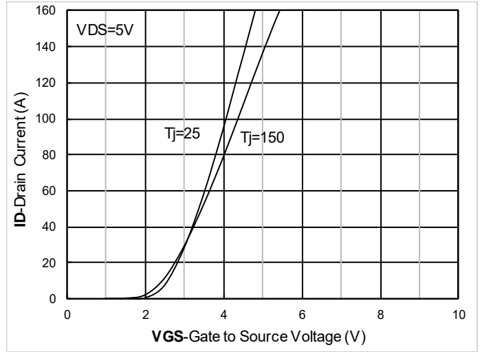
Figure 2. Transfer Characteristics
