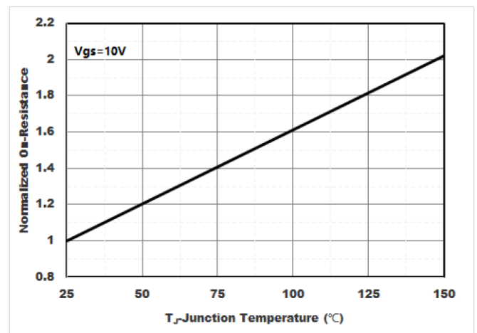
Figure6. Normalized On-Resistance
