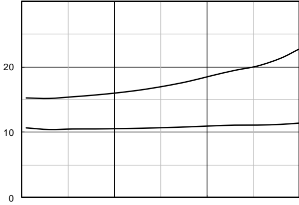
Figure 7. R_{DS(on)} VS Drain Current
